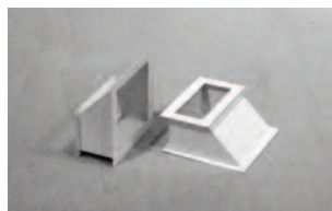
transition piece (for change of cross section) openings 27 1/2 x 27 1/2 and 27 1/2 x 13 3/4 inches (openings 70 x 70 and 70 x 53 cm) PF1767
